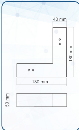
PADUK (180x180x50) mm 111114181380162 Krom Sac (Sheet)
