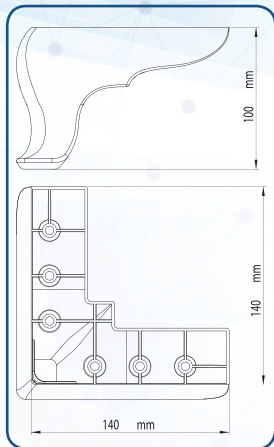
OKALİPTUS (140x140x100) mm 111107112122562 Ağaç
