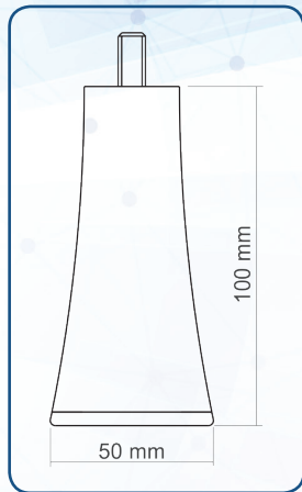
LİMON (100x50) mm 111108501110113 Krom
