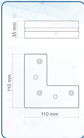
ZEYTİN (110x110x35) mm 121118301122361 Ağaç
