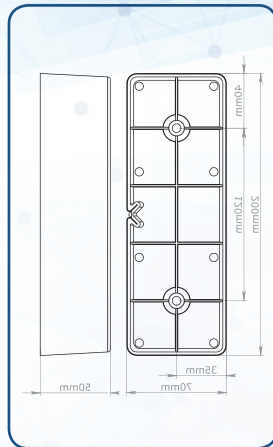
BADEM (70x200x50) mm 111102981380162 Krom Sac (Sheet)
