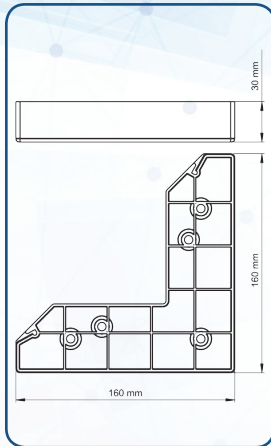
PADUK (160x160x30) mm 111113881380162 Krom Sac (Sheet)
