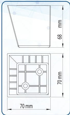
MIMOZA (70x70)mm 111110304353162 Metalik
