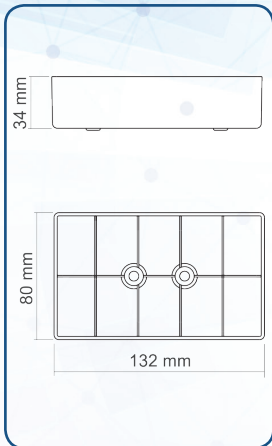
SERVİ (80x132x34) mm 121117204353162 Metalik
