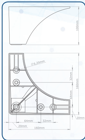
FREZYA (160x160x100)mm 111104501110162 Krom
